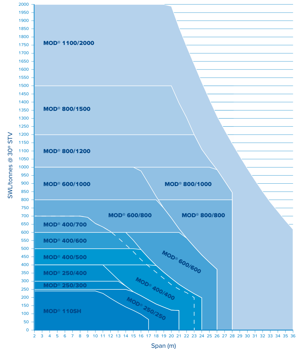
Load v span chart MOD ® 110SH to 1100/2000
