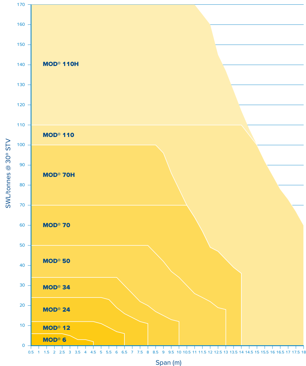
Load v span chart MOD ® 6 to 110H
