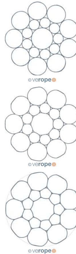
Figure 8: Uncompacted and compacted round strands
