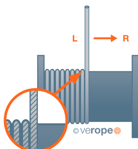
Case C: Overwind: winding direction is from left to right. Left hand lay drums require right hand lay ropes
