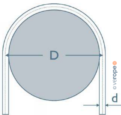
Figure 73: Sheave diameter
