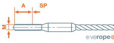
Threaded socket swaged
