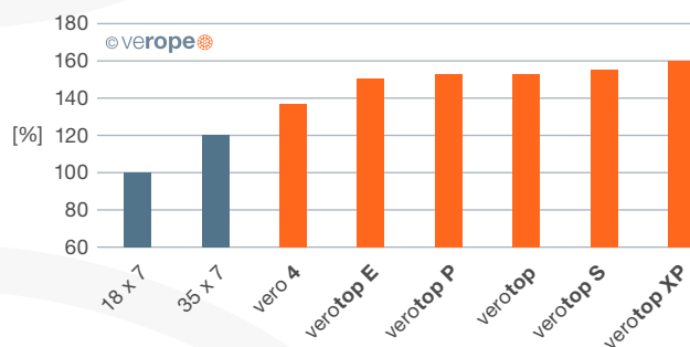
Figure 31: Breaking strengths of rotation-resistant ropes
