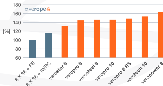
Figure 30: Breaking strengths of non-rotation resistant ropes
