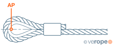
Ferrule-secured eye termination
