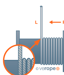
Case D: Overwind: winding direction is from right to left. Right hand lay drums require left hand lay ropes
