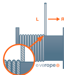
Case B: Unwinding direction is from left to right. Right hand lay drums require a left hand lay ropes
