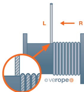
Case A: Unwinding direction is from right to left. Left hand lay drums require right hand lay ropes
